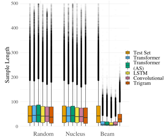
Figure 5: Boxplots showing the distribution of sample length per model and generation scheme. Distribution of test set is repeated in each group for reference.
