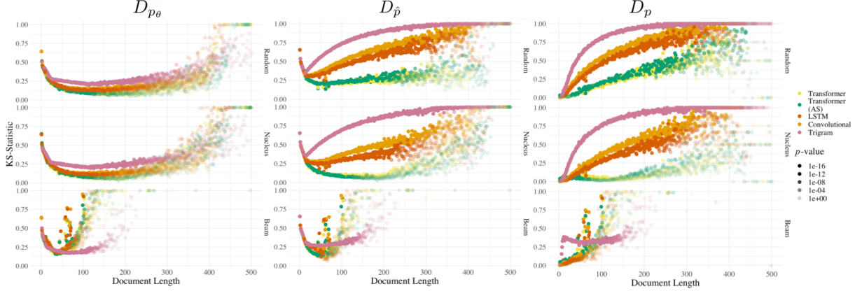
Figure 4: KS metrics (lower implies closer fit) with reference distributions for the type–token relationship as a function of document length. D_{p\theta} and D_{\hat{p}} statistical distance from NHPP distribution for params fit to model text and test sets, respectively; D_p is computed directly against the empirical cdf of test set. Shading indicates significance of the statistic.
