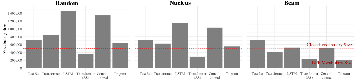
Figure 2: Vocabulary sizes of test set and model-generated samples. Training set (not shown) has vocabulary size of 53.2e5. Only Transformer (AS) and trigram models have a closed vocabulary; the higher red line is the size of the former.
