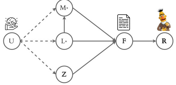
Figure 3: Causal model showing dependencies between the underlying meaning ( U ), lemma ( L_* ) and morpho-syntactic features ( M_* ) of the focus noun, context ( Z ), sentences ( F ) and contextualized representations ( R ).
